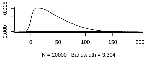
Density of d.l.chemo
