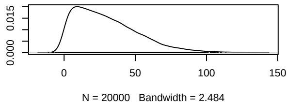
Density of d.III.III_chemo
